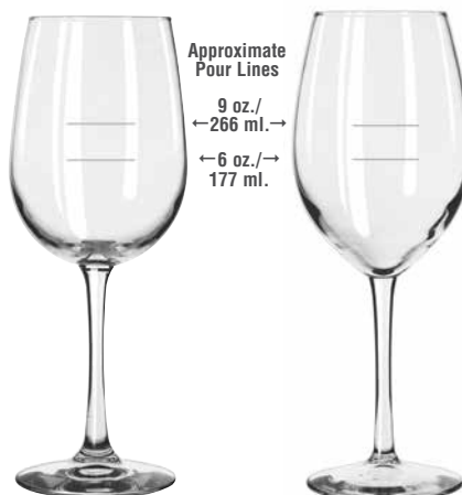
Vina Tall Wine No. 7510-1178N ▲● 16 oz./47.3 cl./473 ml. H9 T2¾ B3¼ D3½ 1 doz./7# • .92 cu. ft. SCC 582713
