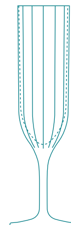
Flute No. 9189 8 oz./23.7 cl./237 ml. H9 T2½ B2¾ D2¾ * SCC 649065
