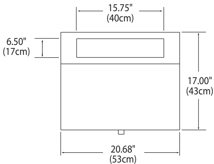
Elevation View
