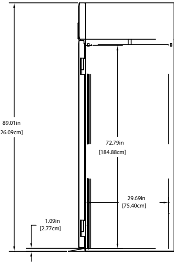
SIDE VIEW ALL MODELS
