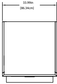
PLAN VIEW ALL 1 SECTION MODELS
