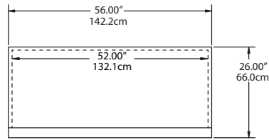
Plan View SSF2S-S, SAF2S-S, SMF2S-S SSF2S-SH, SAF2S-SH, SMF2S-SH
