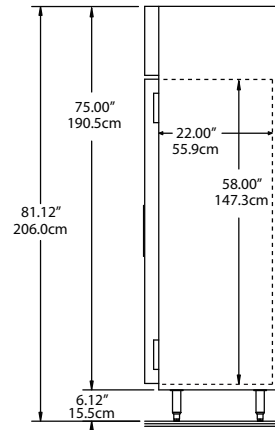
End View All Models
