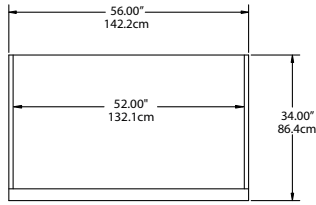
PLAN VIEW SSH2-S, SAH2-S, SMH2-S SSH2-SH, SAH2-SH, SMH2-SH
