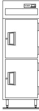
ELEVATION VIEW SSH1-SH, SAH1-SH, SMH1-SH
