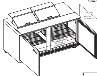
UC4464N-12 ISO View
