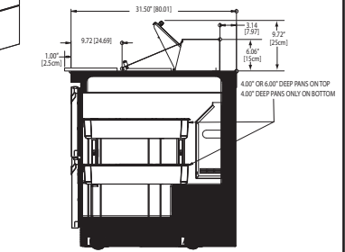
UCD4464N-12 Right Side View
