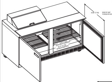
UC4464N-8 ISO View
