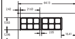
UCD4464N-12 Pan Cutout Configuration
