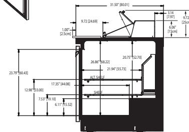
UC4464N-8 Right Side View
