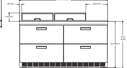
UCD4464N-12 Elevation View
