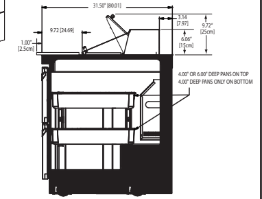
UCD4464N-8 Right Side View
