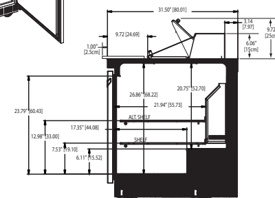
UC4464N-12 Right Side View
