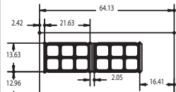
UC4464N-12 Pan Cutout Configuration
