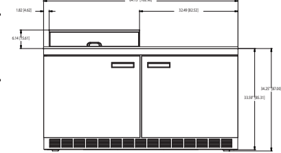
UC4464N-8 Elevation View
