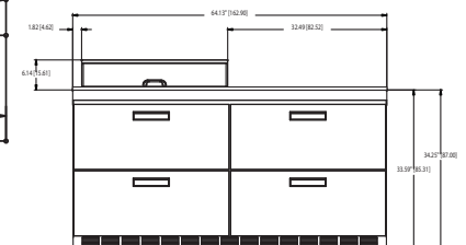
UCD4464N-8 Elevation View
