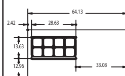
UCD4464N-8 Pan Cutout Configuration
