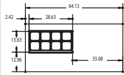
UC4464N-8 Pan Cutout Configuration
