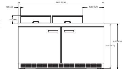
UC4464N-12 Elevation View
