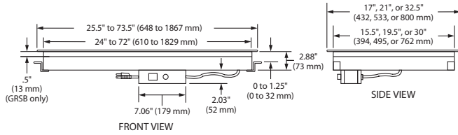
FRONT VIEW SIDE VIEW GRSB Models Shown with Standard Control Box.
