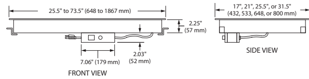
FRONT VIEW SIDE VIEW GRSBF Models Shown with Standard Control Box.
