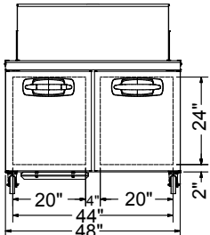
MBSMP48-18A ELEVATION VIEW
