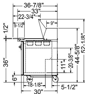
MBSMP48-18A ELEVATION VIEW
