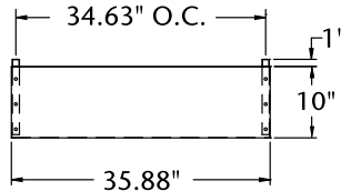
PLAN VIEW MBSP36-10A, MBSMP36-15A
