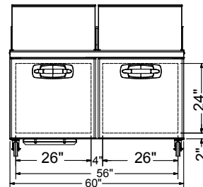
MBSMP60-24A ELEVATION VIEW
