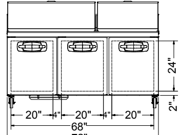
MBSMP72-30A ELEVATION VIEW
