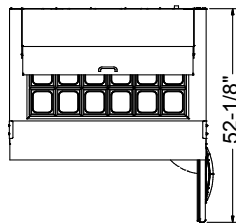
MBSMP48-18A PLAN VIEW
