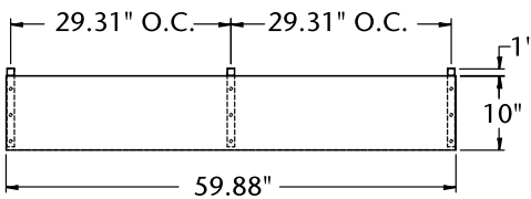
PLAN VIEW MBSP60-16A, MBSMP60-24A
