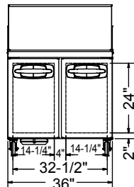
MBSMP36-15A ELEVATION VIEW
