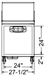
MBSMP27-12A ELEVATION VIEW
