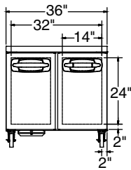
MBUR36A ELEVATION VIEW
