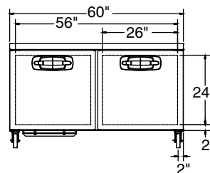
MBUR/MBUF60A ELEVATION VIEW
