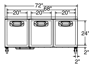
MBUR72A ELEVATION VIEW
