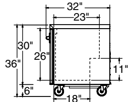
MBUR/MBUF48A ELEVATION VIEW
