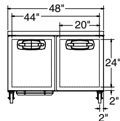
MBUR/MBUF48A ELEVATION VIEW
