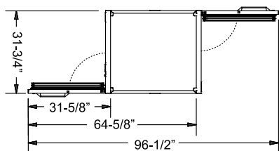
MPWR332 PLAN VIEW
