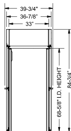
SIDE VIEW - BOTH
