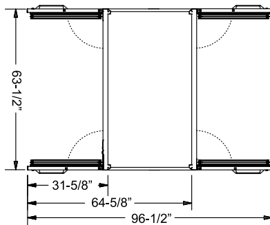
MPWR724 PLAN VIEW
