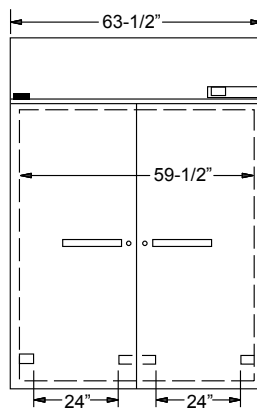
MPWR724 ELEVATION VIEW
