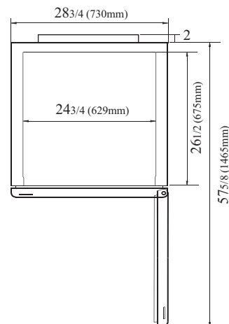
PLAN VIEW
