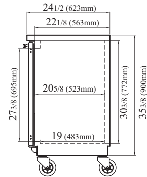
TBB-24-60SG-N SIDE VIEW
