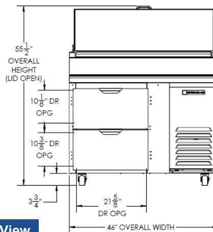
Elevation View
