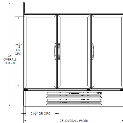
Elevation View
