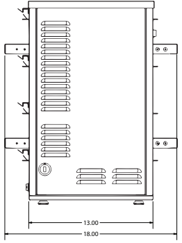
MHG42 with timer bars
