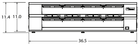
MHG24 with timer bars
