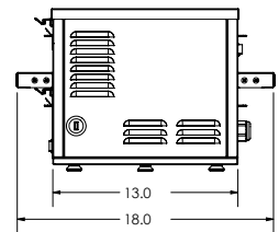
MHG24, MHG23, MHG22 with timer bars
