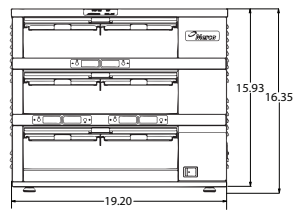
MHG32 with timer bars
