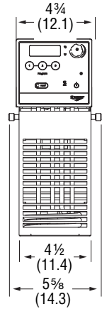
Front View
