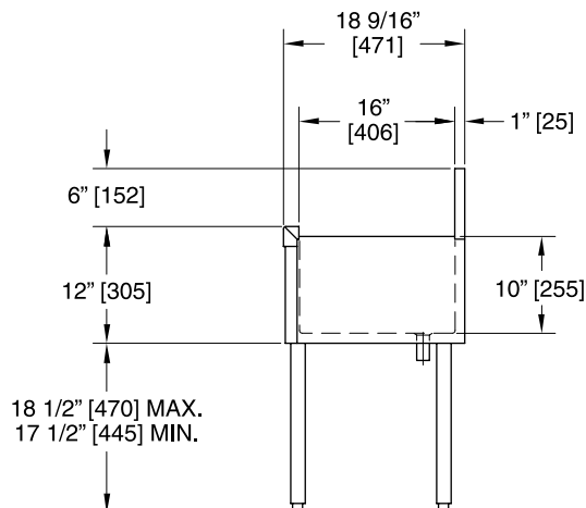
TS END VIEW
