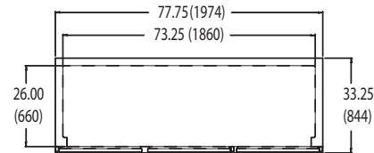
VR-3 TOP VIEW
