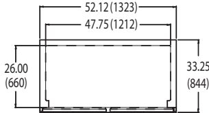
VR-2 TOP VIEW
