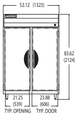
VR-2 FRONT VIEW
