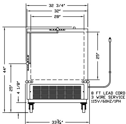
SIDE VIEW (ALL MODELS)
