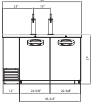
FRONT NLDD59
