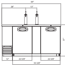
FRONT NLDD69
