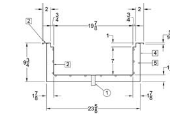
SECTION VIEW SCALE: 1"=1'
