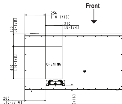
WATER-COOLED
