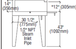
ER-12-5736 SIDE VIEW
