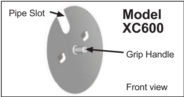
Model XC600 - Air Deflector Plate for Cadco XAF Series Convection Ovens
