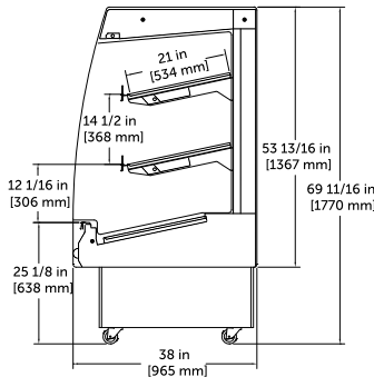
SHELF CONFIG. (3)
