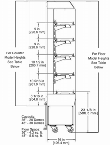
LEFT SIDE VIEW (-V)
