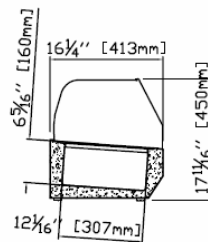
RIGHT VIEW
