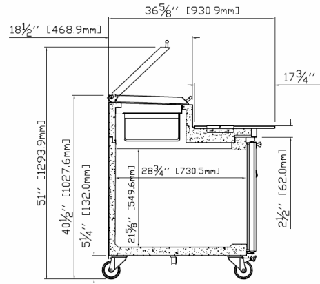
RIGHT VIEW
